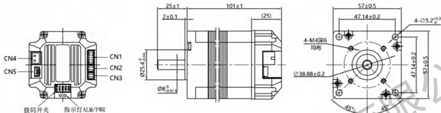
外形图 (DIMENSIONS) unit=mm
