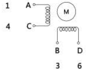
Wiring Diagram
