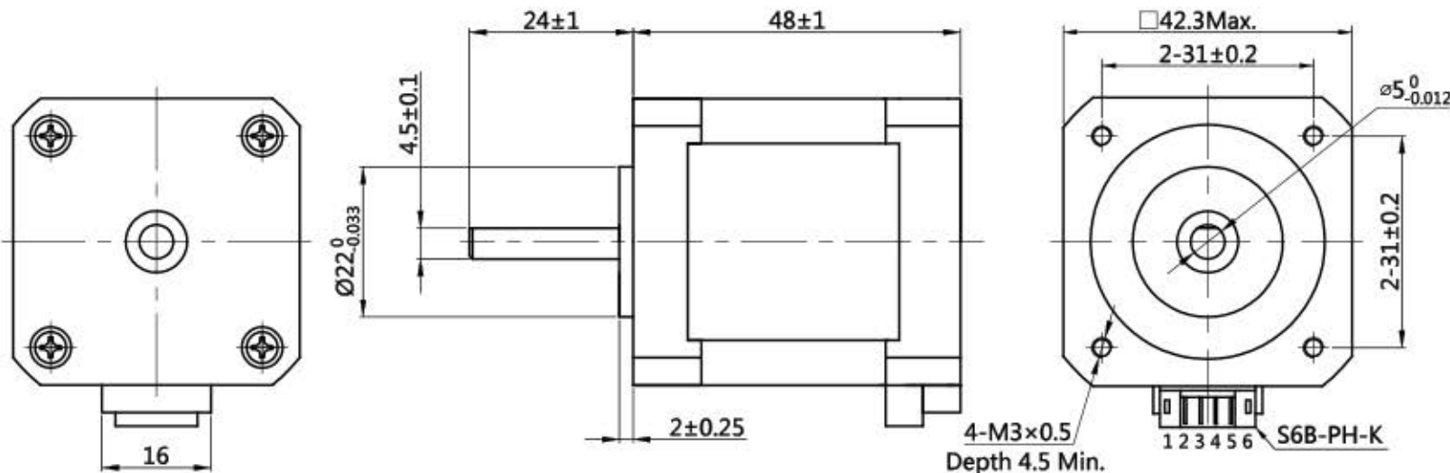
外形图 (DIMENSIONS) unit=mm
