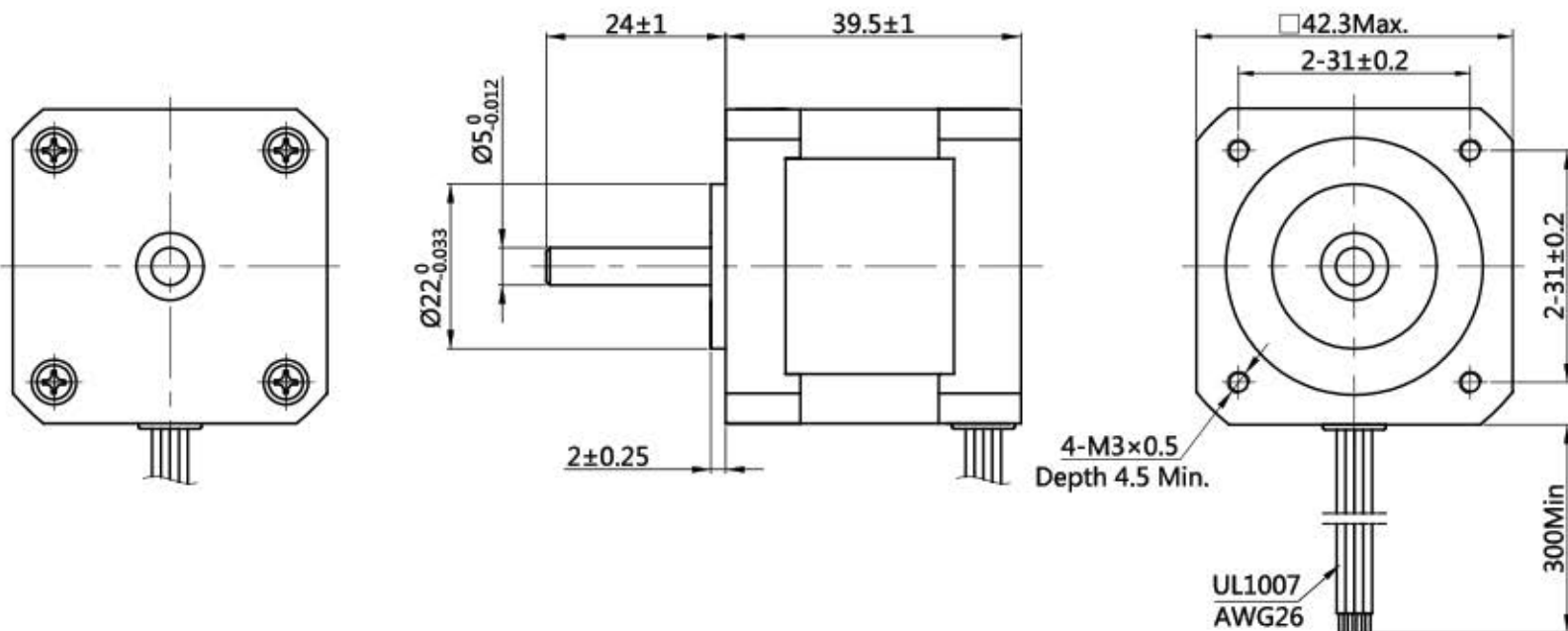
外形图 (DIMENSIONS) unit=mm
